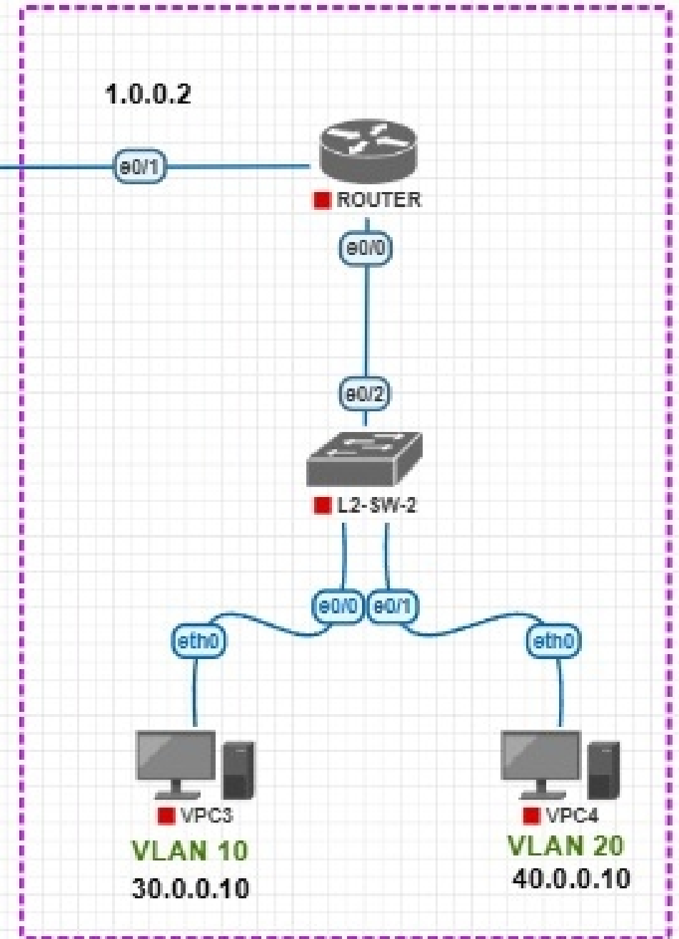
ROUTER ON-A-STICK
